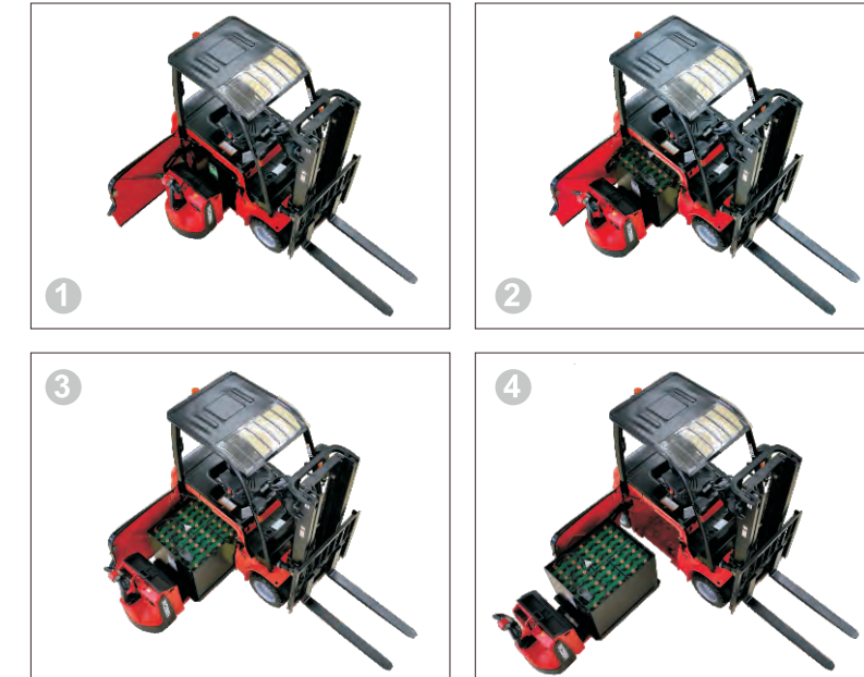
◆ Side access battery. Full opened battery cover (with self-locked spring), easy for battery service.
